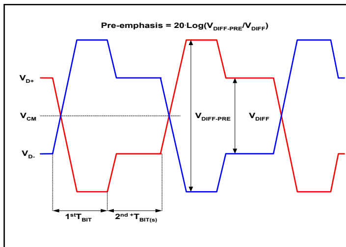
Definition of Pre-emphasis
