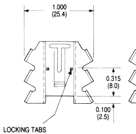
LOCKING TABS 291-C2
