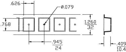
TAPE DETAILS
