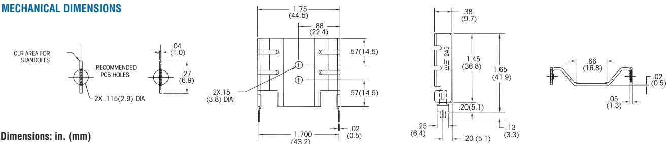
246 SERIES Medium Height, Slim Profile Wavesolderable Folded Fin Heat Sinks
