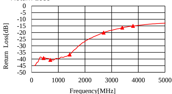
Return Loss
