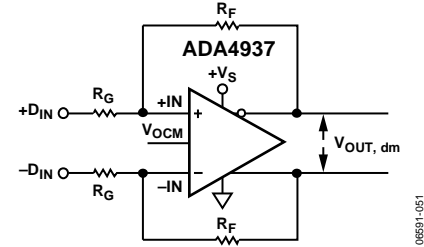
Figure 54. ADA4937-x Configured for Balanced (Differential) Inputs
