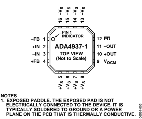
Figure 5. ADA4937-1 Pin Configuration
