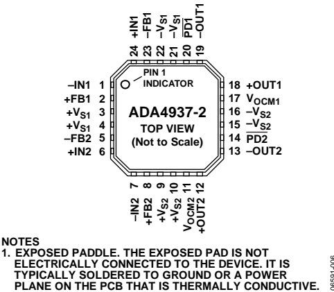
Figure 6. ADA4937-2 Pin Configuration
