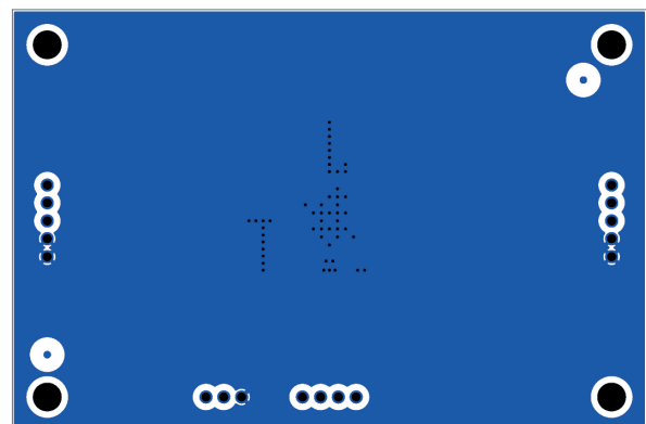
Bottom (GND)
