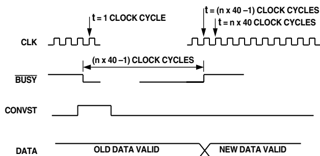
Figure 3. Busy Pulse Timing
