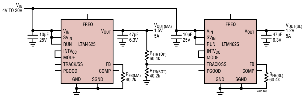
Figure 5. Example Schematic of Ratiometric Output Voltage Tracking
