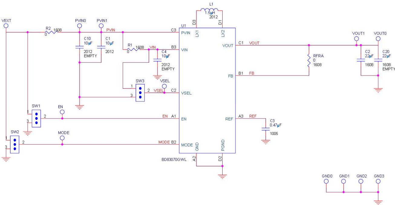
Figure 2. BD83070GWL Evaluation Board Schematic
