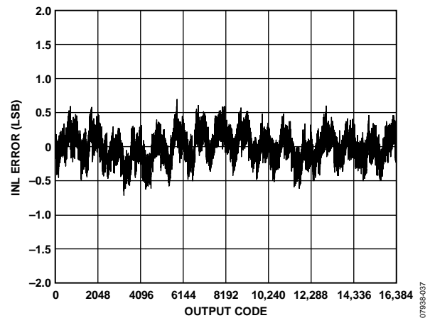
Figure 17. INL Error with f_{IN} = 9.7 MHz
