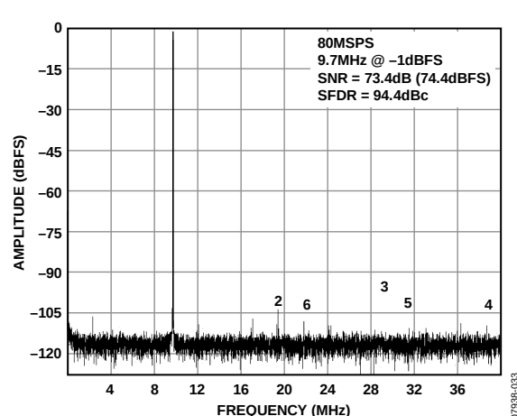
Figure 6. Single-Tone FFT with f_{IN} = 9.7 MHz
