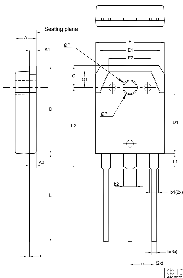
Figure 14. TO3P-3L package outline
