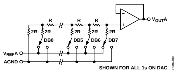
Figure 10. Digital-to-Analog Simplified Circuit Diagram
