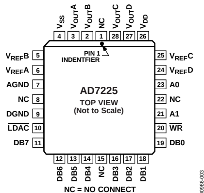
Figure 3. PLCC
