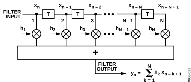
Figure 21. Transversal Filter
