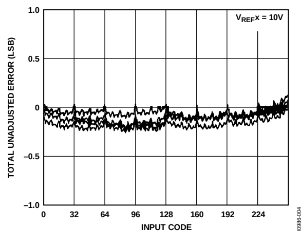
Figure 4. Channel-to-Channel Matching
