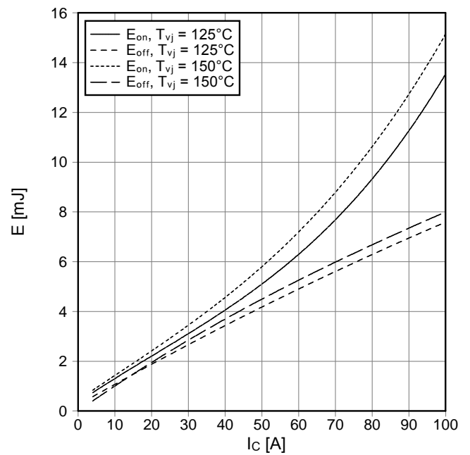
Schaltverluste IGBT-Wechselr. (typisch) switching losses IGBT-inverter (typical) E_{on} = f(I_C), E_{off} = f(I_C) V_{GE} = \pm 15\text{ V}, R_{Gon} = 15\ \Omega, R_{Goff} = 15\ \Omega, V_{CE} = 600\text{ V}
