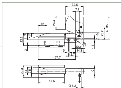
DPNO with lock-on
