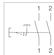
DPNO with lock-off
