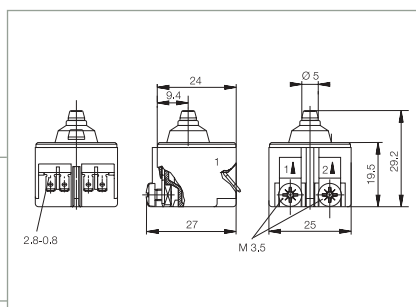
single pole
