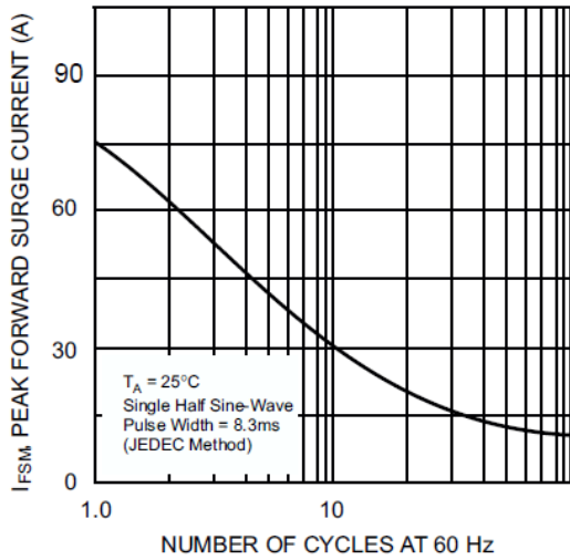
I_{FSM} , PEAK FORWARD SURGE CURRENT (A) NUMBER OF CYCLES AT 60 Hz Fig. 3 Maximum Peak Forward Surge Current (per leg)
