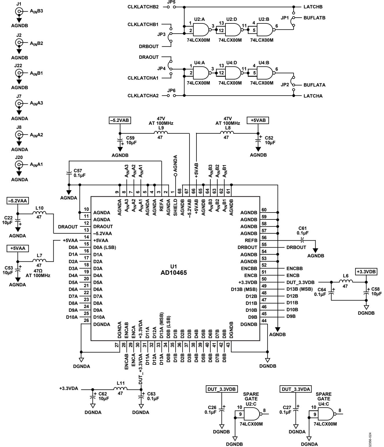
Figure 24. Evaluation Board
