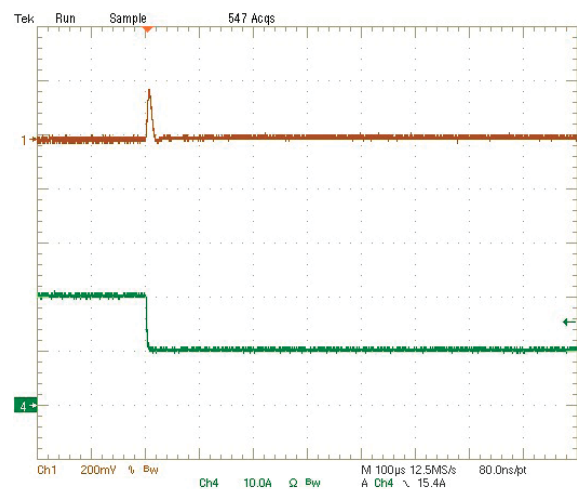
Step Load Transient Response (Vin=5.0V, Vout=2.5V, Cload=94μF, Iout=20A to 10A) Trace 1=Vout, 200 mV/div, Trace 4=Iout, 10A/div.
