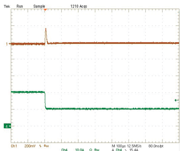
Step Load Transient Response (Vin=5.0V, Vout=3.3V, Cload=94μF, Iout=20A to 10A) Trace 1=Vout, 200 mV/div, Trace 4=Iout, 10A/div.
