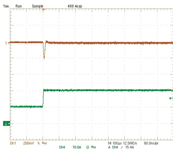
Step Load Transient Response (Vin=5V, Vout=1.2V, Cload=94μF, Iout=6A to 12A) Trace 1=Vout, 200 mV/div, Trace 4=Iout, 10A/div.
