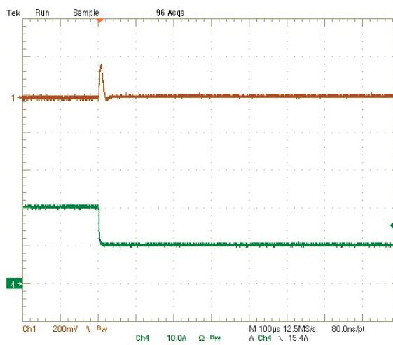
Step Load Transient Response (Vin=5.0V, Vout=1.2V, Cload=94μF, Iout=20A to 10A) Trace 1=Vout, 200 mV/div, Trace 4=Iout, 10A/div.
