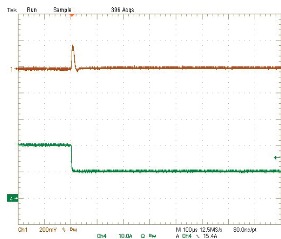
Step Load Transient Response (Vin=5V, Vout=1.2V, Cload=94μF, Iout=20A to 10A) Trace 1=Vout, 200 mV/div, Trace 4=Iout, 10A/div.
