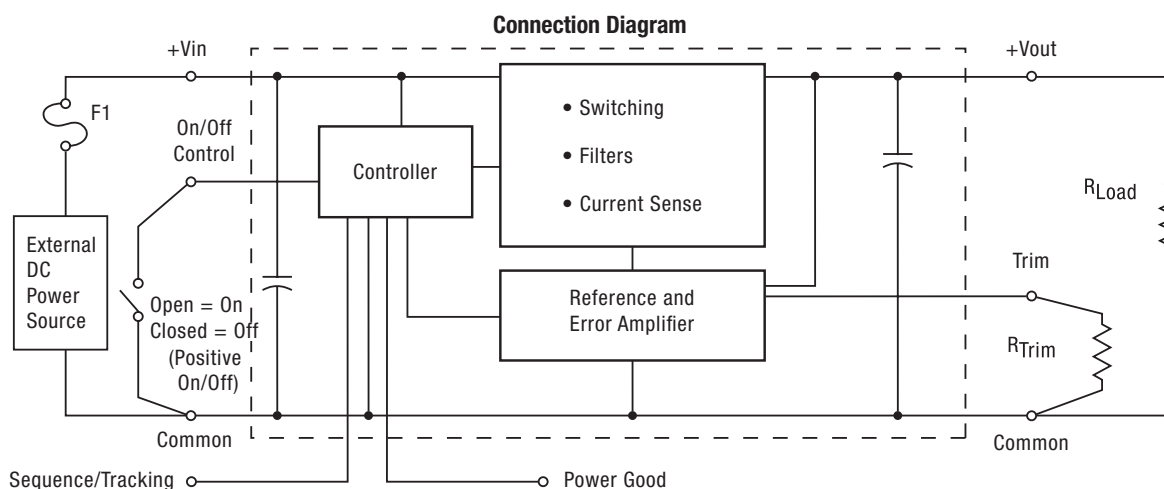
Figure 1. OKL2-T/20-W5
