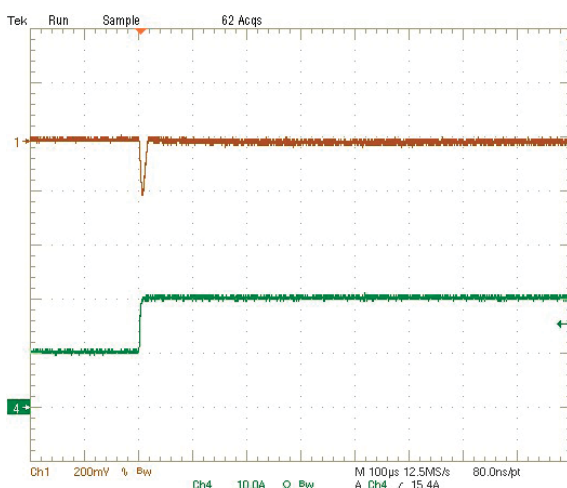
Step Load Transient Response (Vin=5.0V, Vout=3.3V, Cload=94μF, Iout=6A to 12A) Trace 1=Vout, 200 mV/div, Trace 4=Iout, 10A/div.
