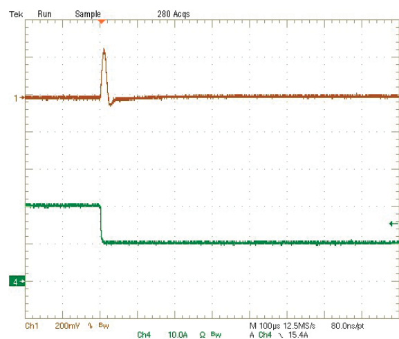
Step Load Transient Response (Vin=5V, Vout=0.6V, Cload=94μF, Iout=20A to 10A) Trace 1=Vout, 200 mV/div, Trace 4=Iout, 10A/div.
