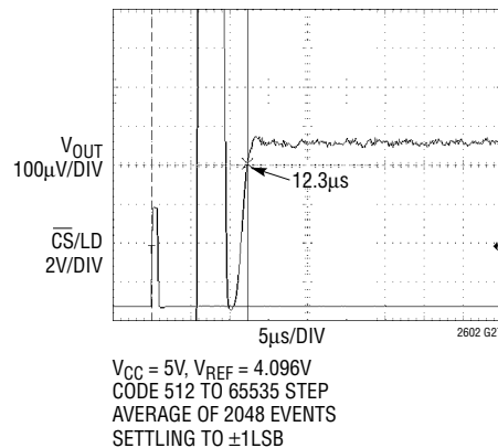
Settling of Full-Scale Step
