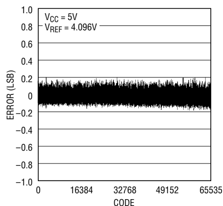
Differential Nonlinearity (DNL)(LTC2602)
