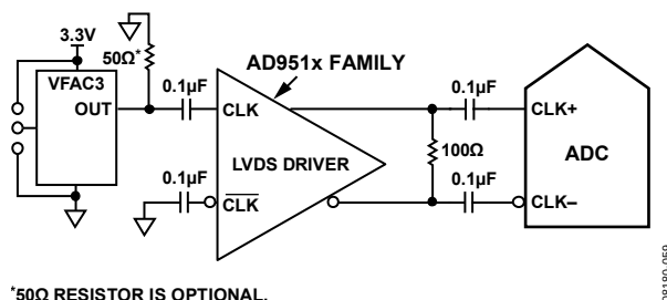
Figure 65. Differential LVDS Sample Clock
