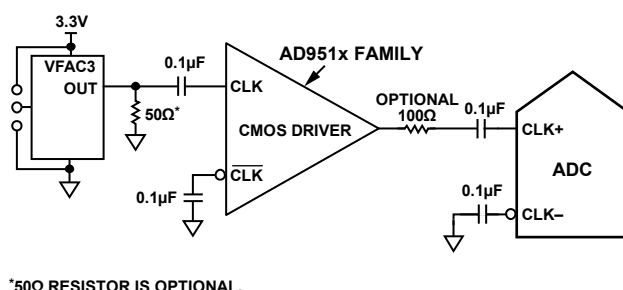
Figure 67. Single-Ended 3.3 V CMOS Sample Clock
