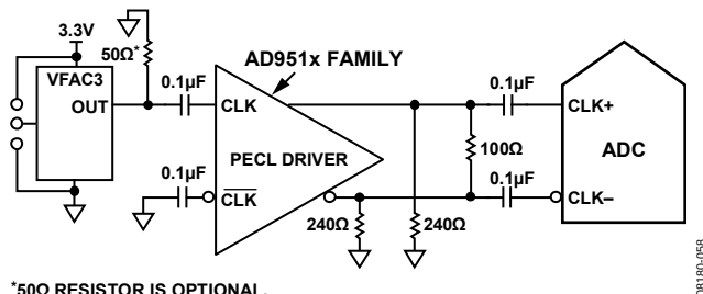
Figure 64. Differential PECL Sample Clock
