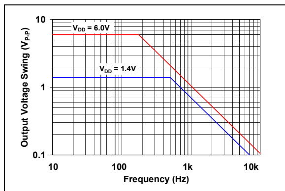
FIGURE 2-21: Output Voltage Swing vs. Frequency.
