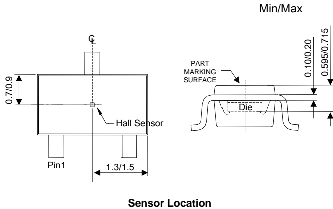
Sensor Location
