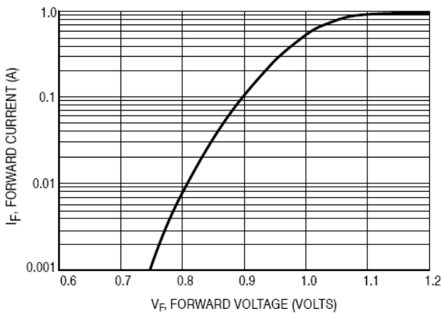
Figure 5. Forward Voltage
