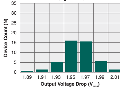
Typical On-State Output Forward Voltage Distribution ( T_A=25^\circ C )
