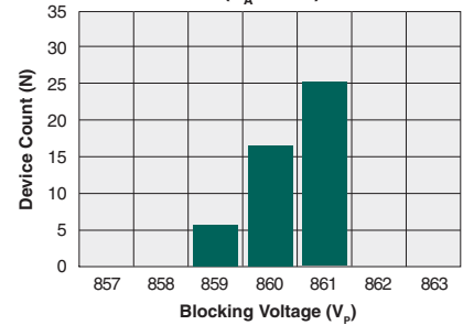
Typical Blocking Voltage Distribution ( T_A=25^\circ C )
