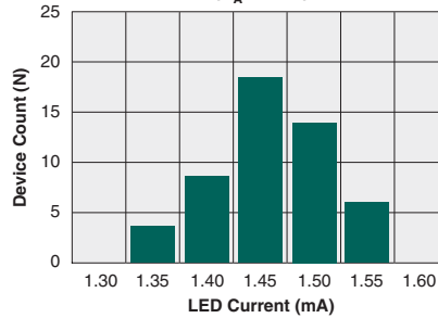
Typical I_F for Switch Operation ( T_A=25^\circ C )
