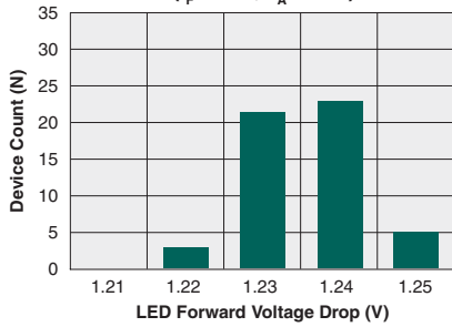
Typical LED Forward Voltage Drop ( I_F=5mA, T_A=25^\circ C )
