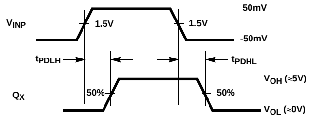
FIGURE 4. t_{PD} RECEIVER PROPAGATION DELAY MEASUREMENT POINTS
