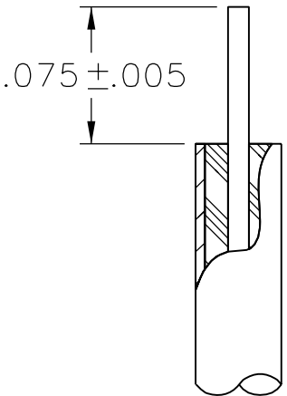
CABLE STRIP DIMENSIONS 10:1
