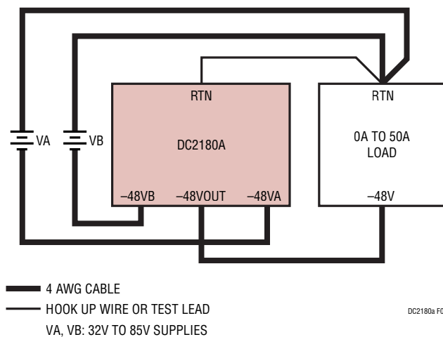
Figure 1. Test Setup
