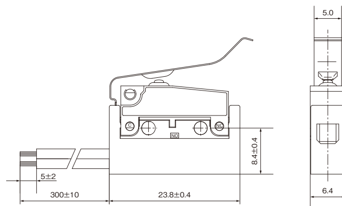
Wire leads left angle type
