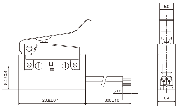
Wire leads right angle type
