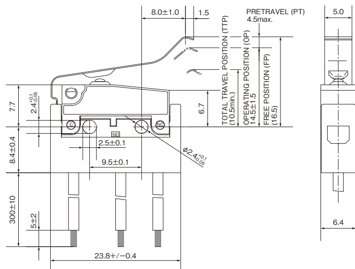
Wire leads left angle type
