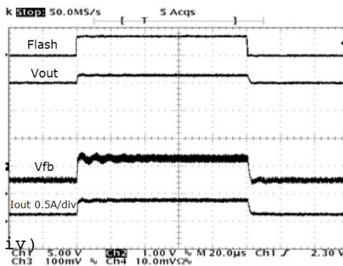
Fig. 20: Torch in 1x Mode V_{IN}=4.2V , C_{IN}=4.7\mu F , C_{FC}=0.47\mu F , C_{OUT}=2.2\mu F
