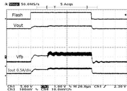
Fig. 21: Torch in 1x Mode V_{IN}=3.6V , C_{IN}=4.7\mu F , C_{FC}=0.47\mu F , C_{OUT}=2.2\mu F
