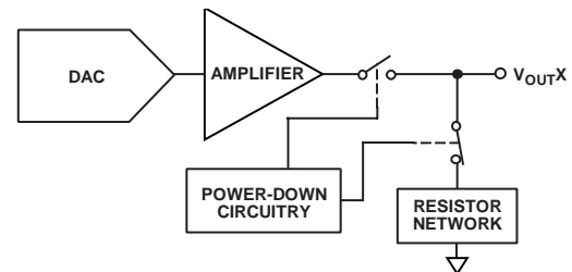
Figure 45. Output Stage During Power-Down
