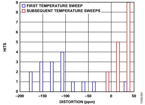
Figure 49. Thermal Hysteresis
