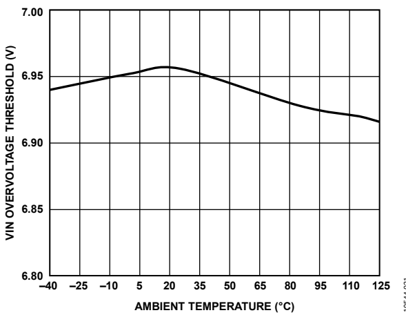
Figure 21. VINx Overvoltage Threshold vs. Ambient Temperature
