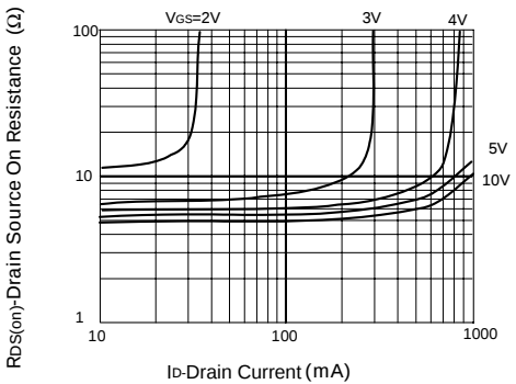
On-resistance v drain current
