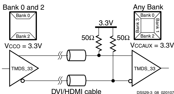
Figure 8: External Input Resistors Required for TMD5 33 I/O Standard
