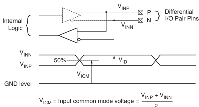
Figure 4: Differential Input Voltages
