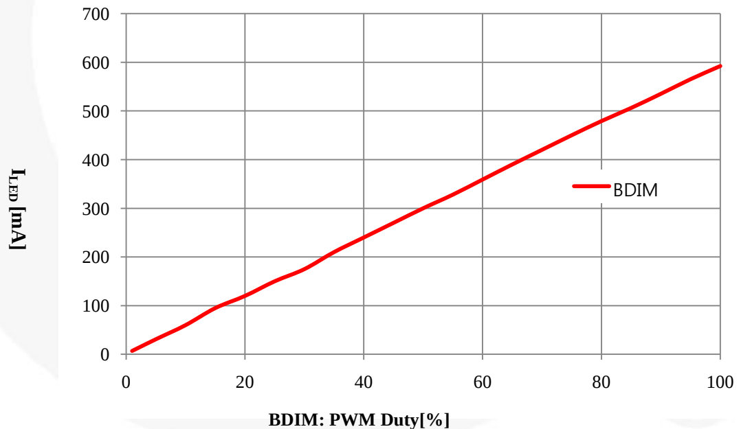
Figure 70. PWM Characteristics
