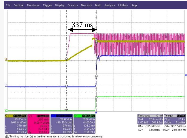
Figure 34. V IN = 300 V AC / 50 Hz
