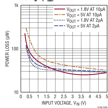
Light Load Power Loss vs Input Voltage ( V_{IN} )
