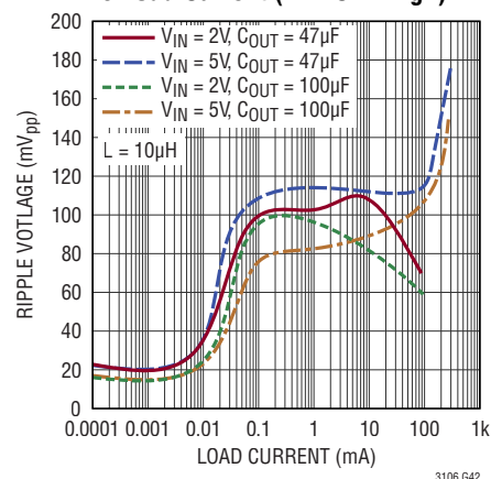
5V Output Voltage Ripple vs Load Current ( I_{LIMSEL} High)
