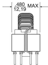
P0584 (6 pins)
