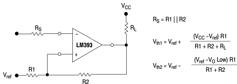
Figure 12. Comparator with Hysteresis
