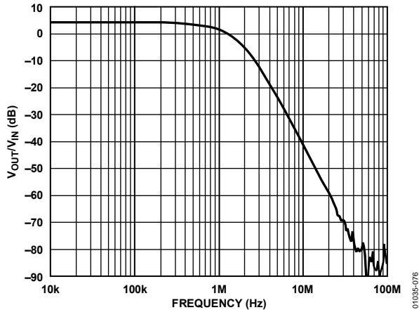
Figure 78. Frequency Response of 1 MHz Low-Pass Filter
