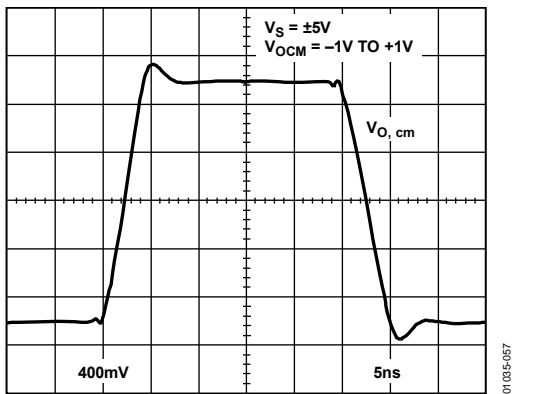
Figure 49. V_{OCM} Transient Response
