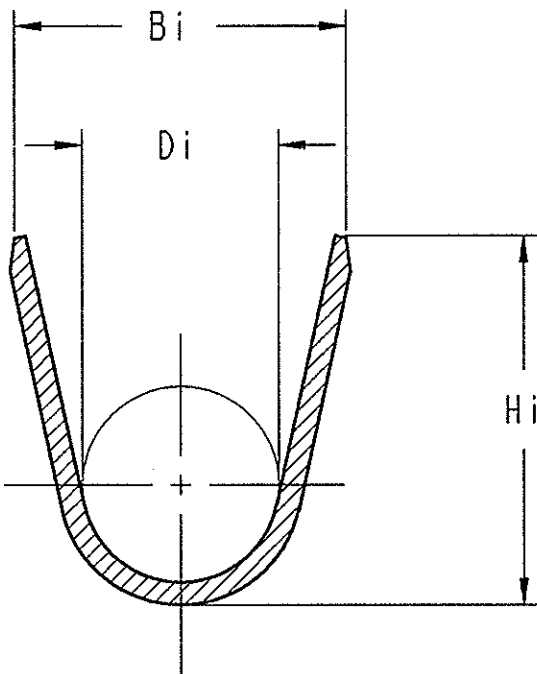
SECTION B-B
