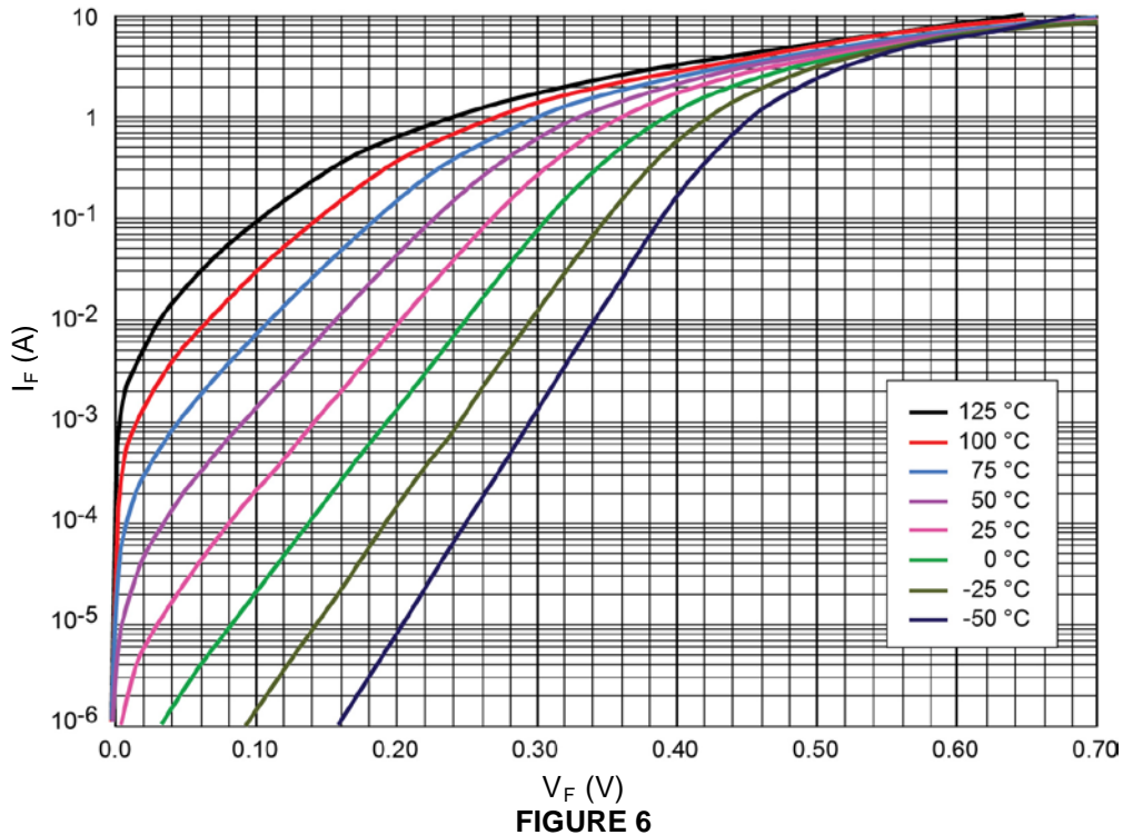
FIGURE 6 Schottky V_F - I_F Characteristics (Typical 1N6864)
