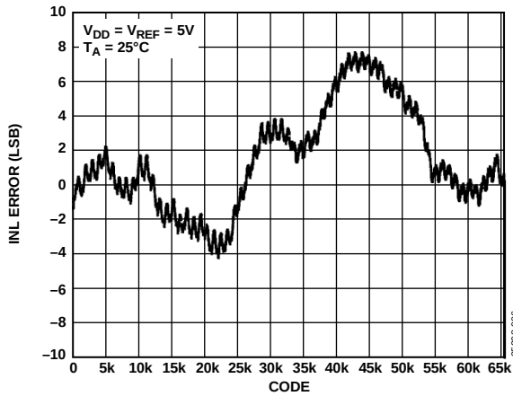
Figure 6. INL
