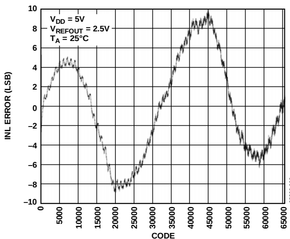
Figure 8. INL—AD5666-2
