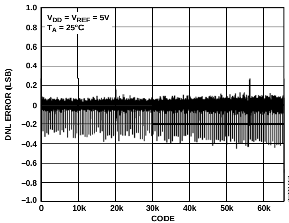
Figure 7. DNL
