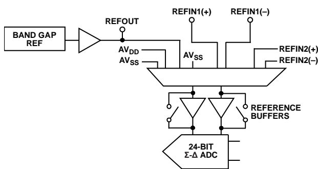
Figure 75. Reference Connections
