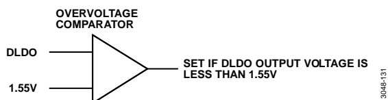
Figure 121. Digital LDO Monitor
