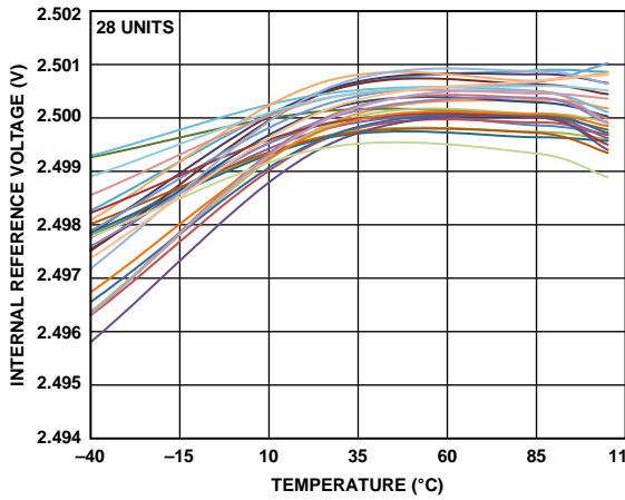
Figure 29. Internal Reference Voltage vs. Temperature
