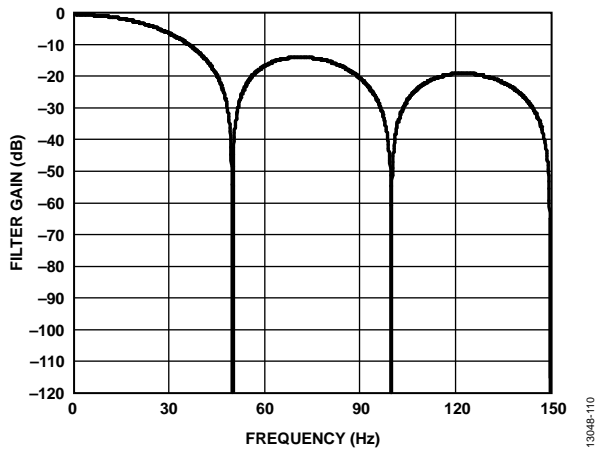
Figure 100. 50 Hz Rejection
