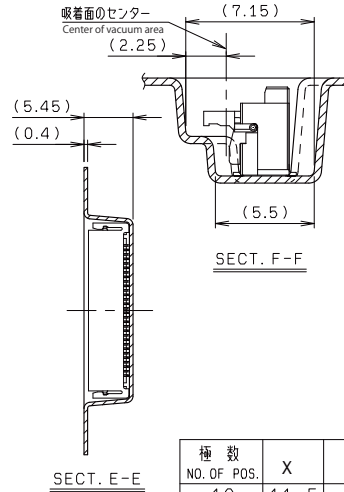
SECT. E-E
