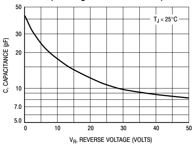
Figure 5. Typical Capacitance
